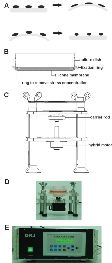
Figure 1 (a) Strain cell theory. Cells were stretched when the membrane was expanded since the cells were seeded on the relaxed membrane and compressed when the membrane was relaxed. (b) The force-loading dishes with the bottom part of the cell culture dishes replaced with a medical silicone membrane. (c) The carrier rod was driven by a hybrid motor. (d) The cell culture dish was fixed above the carrier rod to accomplish cell compression or stretching. (e) A central processing unit was used to control the hybrid motor precisely with the prescription programming.
