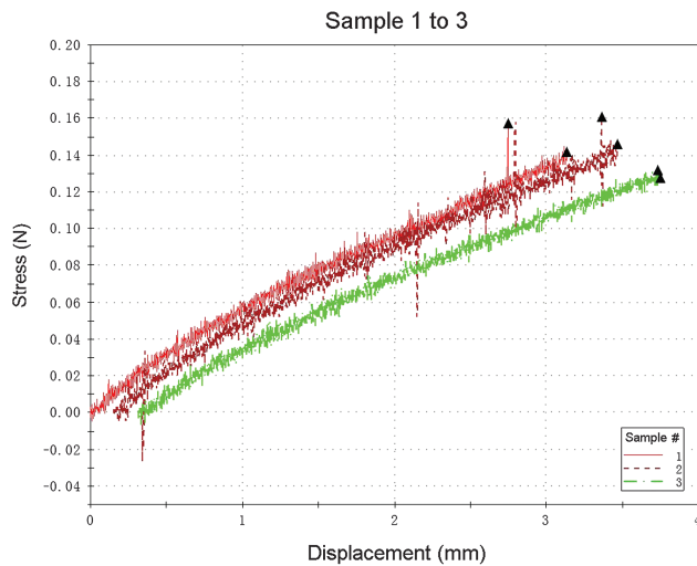
Figure 2 Stress-strain curves were linear with almost the same slope in three randomly selected regions of the membrane.
